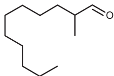
Undecanal, 2-methyl-
